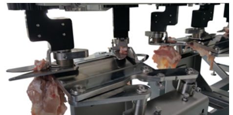
Tendon and muscle cutting assembly
